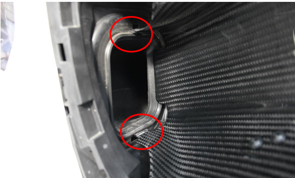
19. The clips on the top and bottom of the scoop should go into the openings on the duct.
