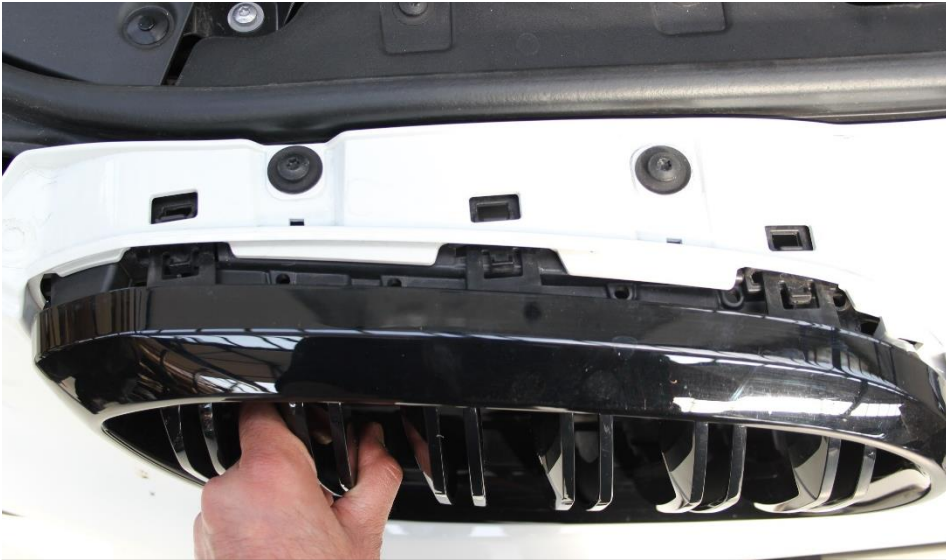
13. Remove the grills – push the tabs in on the top while pulling to release them.
